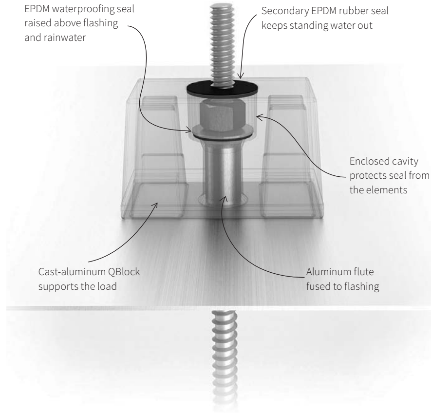
Classic Comp Mount
